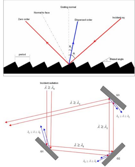
Figure 3: Top: Zeroth-order and first-order diffraction at a blazed grating. Bottom: A multichannel spectrograph consisting of three reflection gratings.
